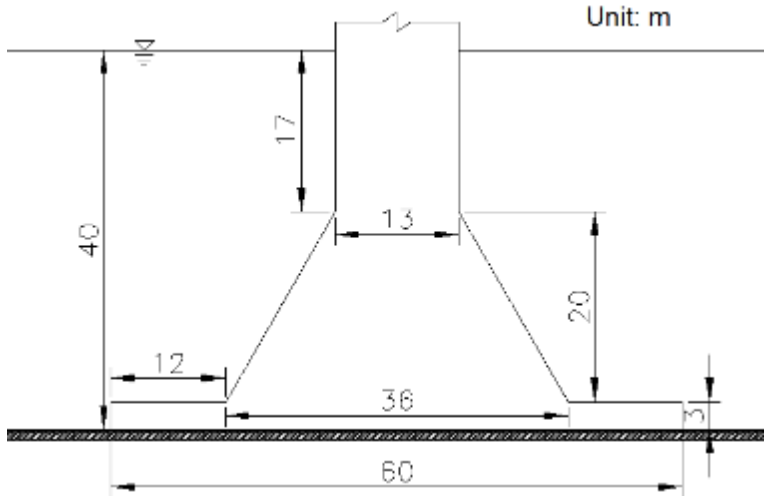
Figure. 4 GBS foundation in water depth of 40 m
