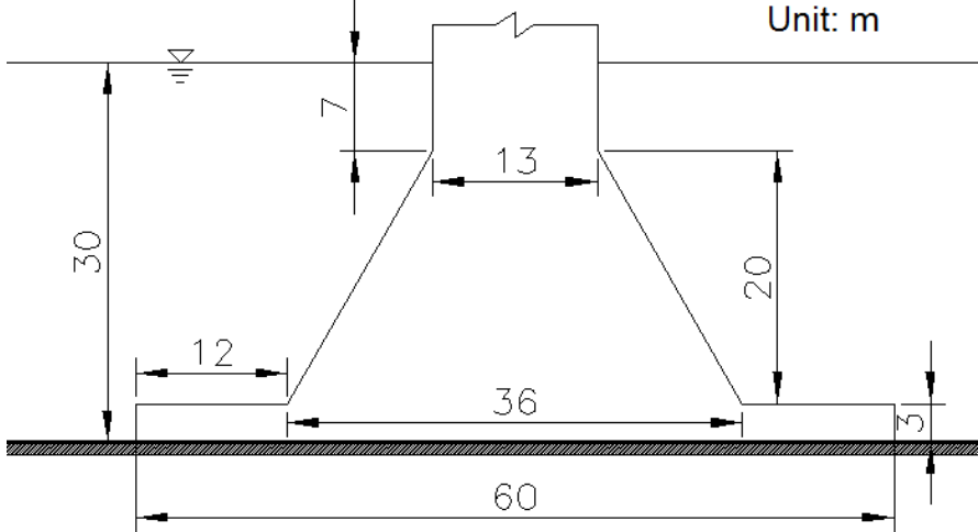
Figure 2 GBS foundation in water depth of 30 m
