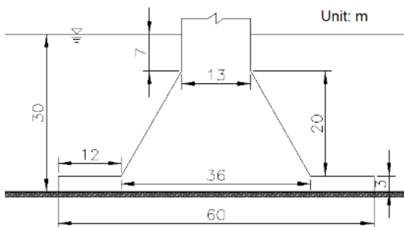
Plate 3.1: GBS dimensions for 19MW wind turbines (here shown in 30m water depth)
