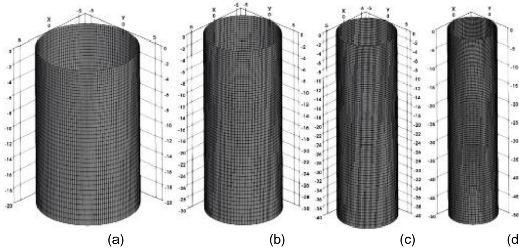
Figure 13 Numerical mesh for monopile #2 (D =12m) in different water depths (a) 20m (b) in 30m (c) in 40m (d) in 50m
