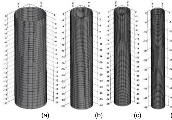
Figure 12 Numerical mesh for monopile #1 (D =6.5m) in different water depths (a) 20m (b) 30m (c) 40m (d) 50m
