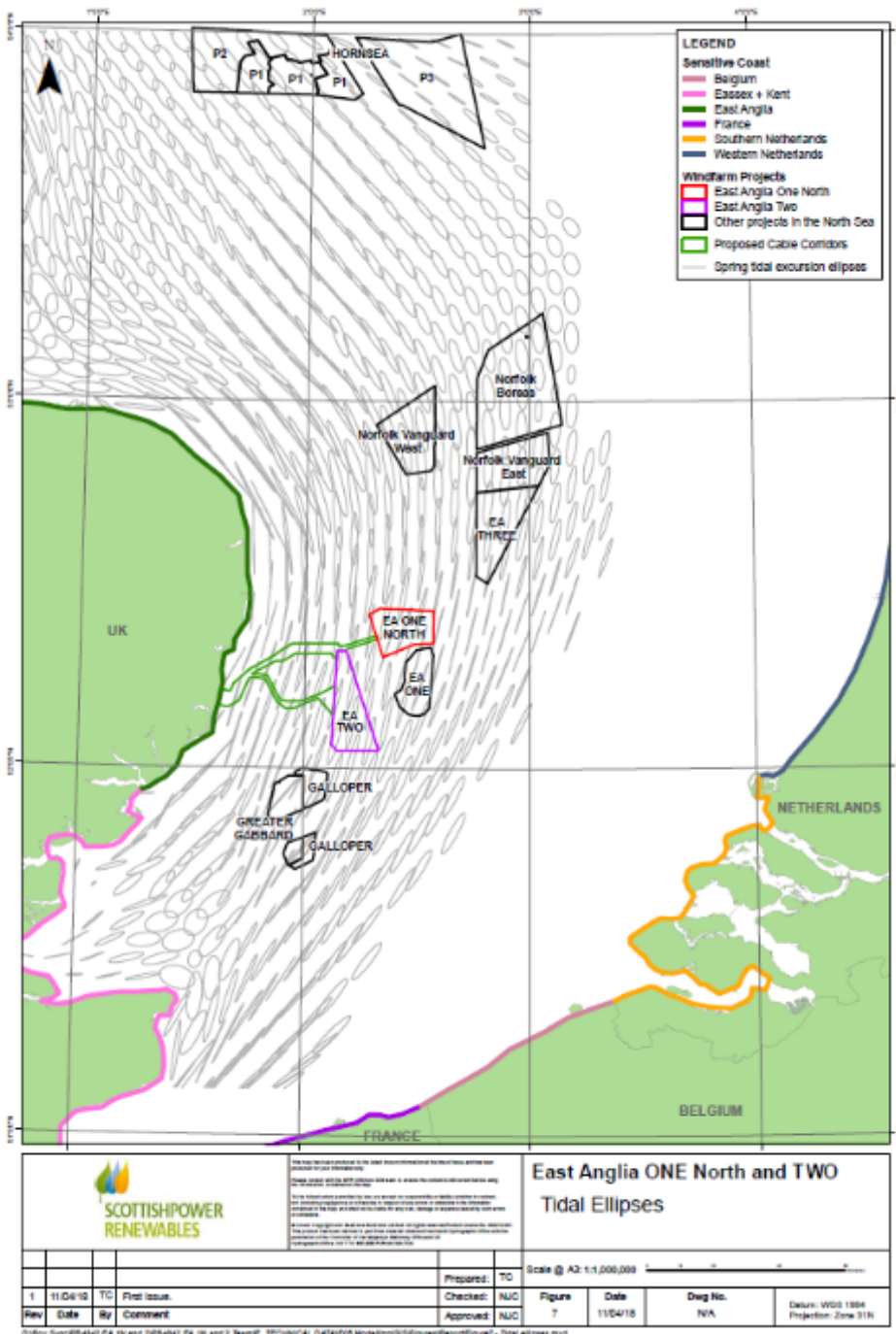
Figure 7: Tidal ellipses
