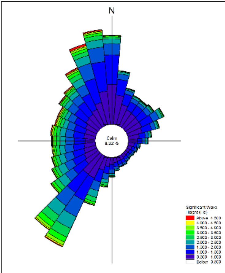
Figure 1: Offshore wave rose
