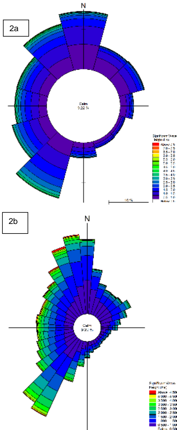
Figure 2a & b: Wave rose of hindcase model data
