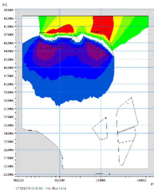
Plate 4:21: Percentage changes in baseline wave height arising cumulatively from Hornsea Project 1, Project 2 and Project 3 under a 1 in 1 year return period event (waves from NNE)
